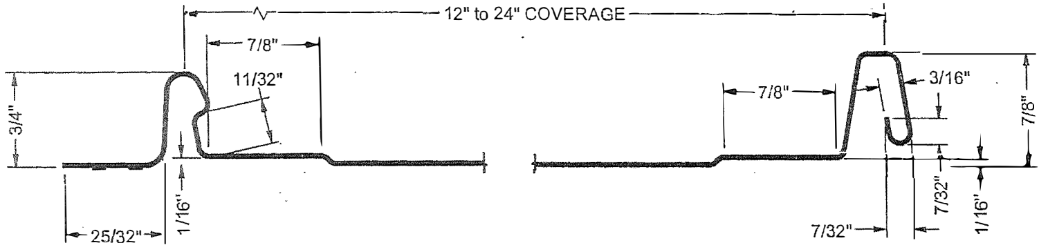
DETAIL A
